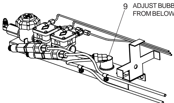
Dual Valve Assy. (Item 28) W/Regulator P/N 98837C For Use On Models 4420BF1LDBFR and 4420BF1UDBFR (Tubing Not Included)
