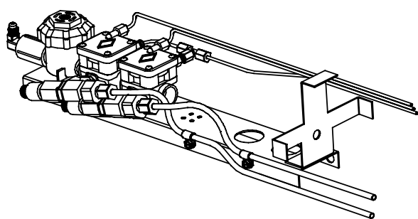
Dual Valve Assy. (Item 27) W/O Regulators P/N 98838C For Use On Models 4420BF2DBFR (Tubing Not Included)
